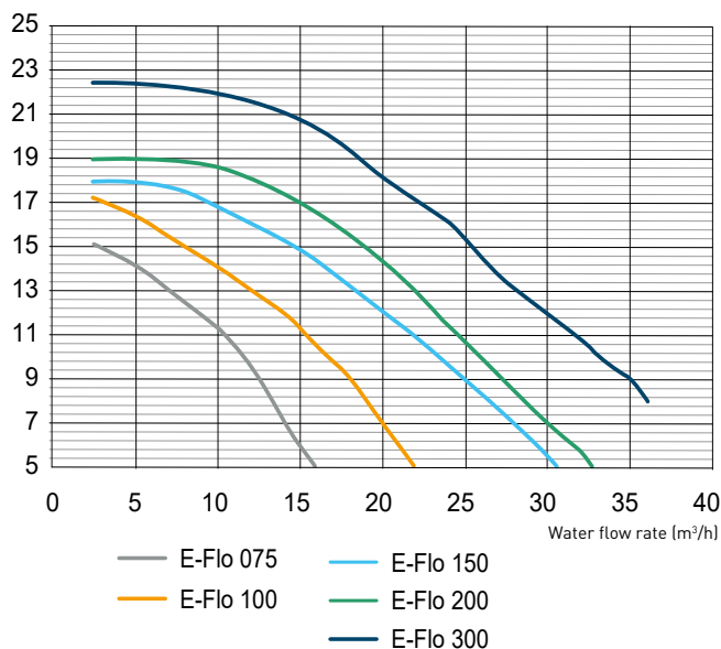
Water column pressure (m) E-Flo
